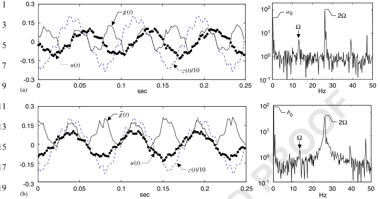
Fig. 9. Typical experimental results at \Omega = 13 Hz: (a) g(t) ; (b) \tilde{g}(t) . The frequency plots are the FFT of the corresponding g(t) .
