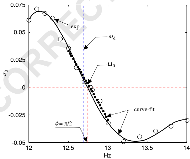
Fig. 10. a_0 at frequencies near \omega_d (○: experiment; — and - -: curve-fitted).
